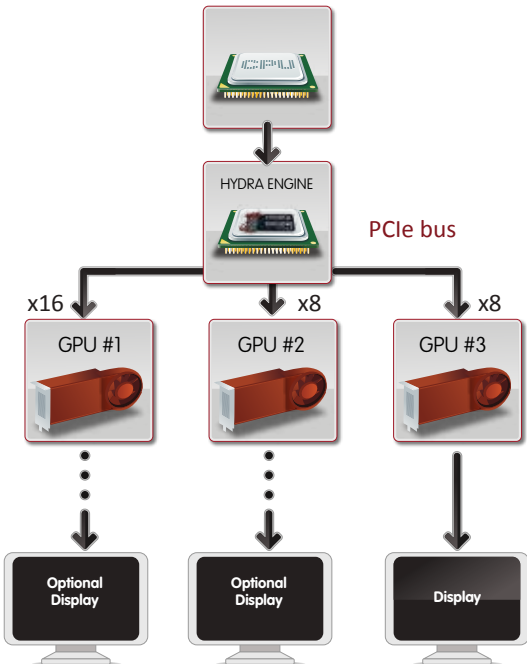
Configuration C - 1 x 16 + 2 x 8 downstream ports
