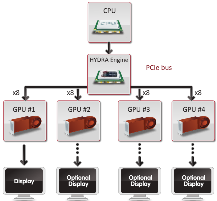
Configuration B - 4 x 8 downstream ports
